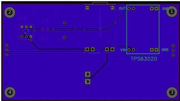
PCB Layout - Bottom Side
